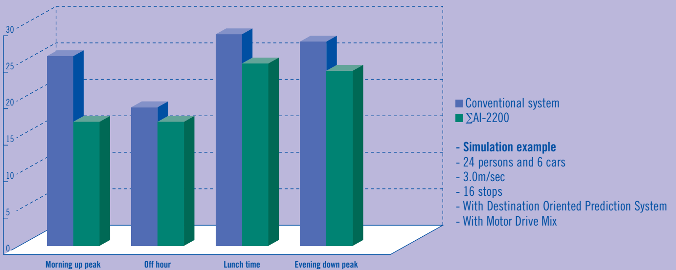
- \Sigma AI-2200 Performance: Average waiting time (sec.)
